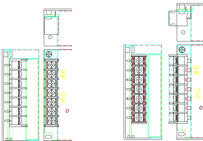
Type A: Stright pins with pc cover
